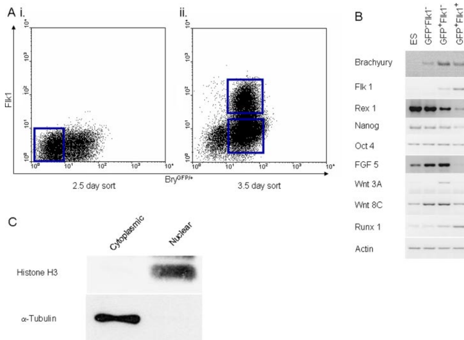
FIG. 1. Enrichment of ES cells at specific stages of development for nuclear proteomics analysis and comparison with transcriptome data. A , flow cytometric enrichment of Bry GFP/+ ES cells based on GFP and Flk1 expression. At least 20 million cells were prepared for each experiment by flow cytometric sorting. i. , scatter plot of data from time point 2.5 days after LIF withdrawal and cells being placed in suspension culture to promote embryoid body formation; the blue gate shows the GFP - Flk1 - cells. ii. , cells after 3.5 days without LIF showing the upper and lower blue gates set for collection of GFP + Flk1 - and GFP + Flk1 + cells, respectively. Results are from one of three experiments where cells were taken for proteomics and transcriptomics analysis. B , gene analysis of the four populations of cells. RNA was extracted from unsorted Bry GFP/+ ES cells and sorted differentiated cells. Semiquantitative RT-PCR was carried out on genes known to be involved in Bry GFP/+ ES cell differentiation. C , Western blot analysis of known nuclear and cytosolic proteins in fractions prepared from ES cells. Bry GFP/+ ES cells were lysed and fractionated, and a nuclear fraction was prepared. Western blot analysis for a cytosolic ( \alpha -tubulin) and a nuclear (histone H3) protein was performed to assess nuclear preparation enrichment. Results shown are typical of four fractionation experiments performed.
