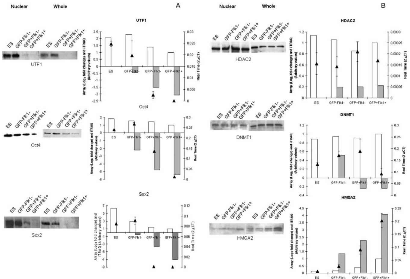
FIG. 5. A comparison of relative expression levels of proteins and mRNA validated with the use of real time PCR and Western blot. A, Oct4, UTF1, and Sox2, known regulators of pluripotency, were identified in our proteomics and microarray analysis and validated with the use of Western blot and real time PCR, respectively. B, validation of the protein and mRNA expression levels of HMGGA2, HDAC2, and DNMT1. Western blots were performed with both nuclear and whole cell preparations. The iTRAQ data for each protein is shown (white histogram) with data from real time PCR analysis (line) and microarray (gray histogram). Error bars shown are from three observations and represent the S.E.
